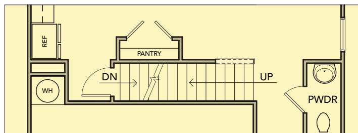
First Floor Plan With Opt. Basement
