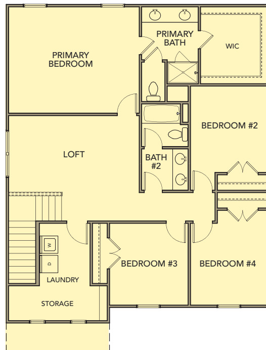
Second Floor
