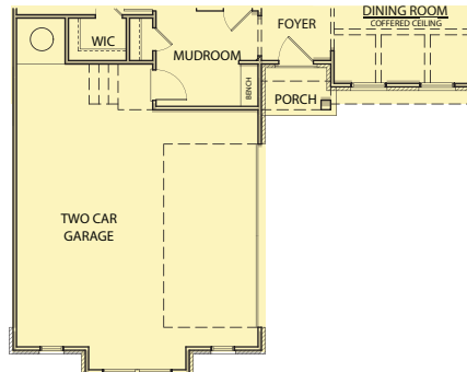
First Floor - FH
