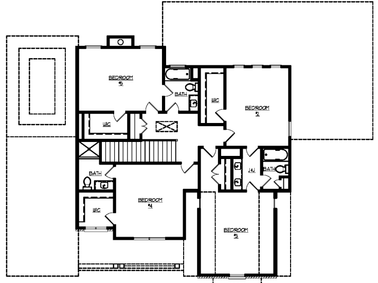
SECOND FLOOR PLAN W/ OPT. BEDROOM #5
