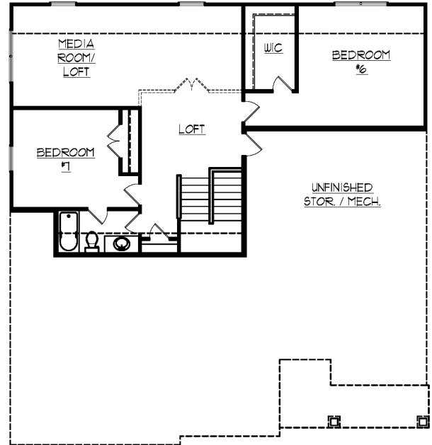
OPT. THIRD FLOOR PLAN
