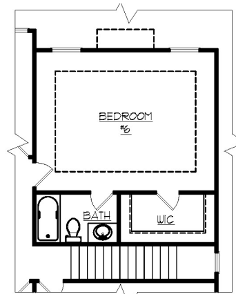
SECOND FLOOR PLAN W/ OPT. BEDROOM #6
