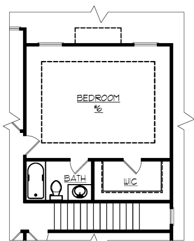
SECOND FLOOR OPTIONAL 6TH BEDROOM
