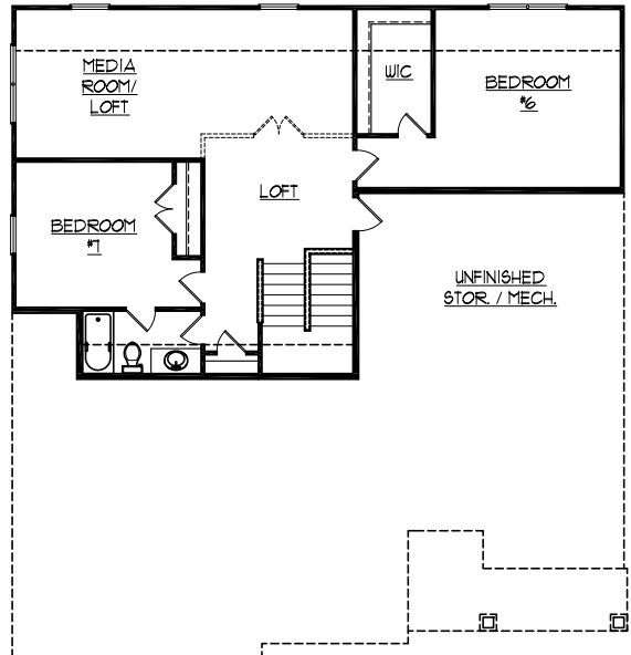
OPT. THIRD FLOOR PLAN
