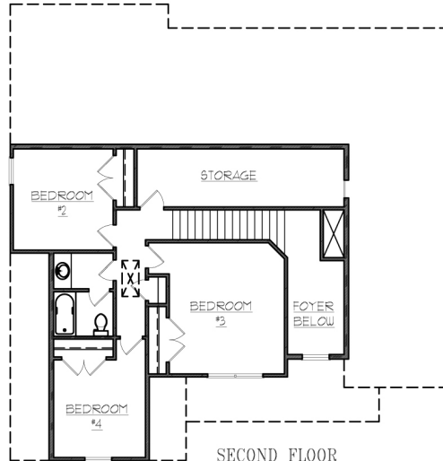
SECOND FLOOR PLAN "STANDARD"
