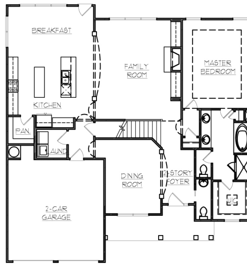
FIRST FLOOR PLAN "STANDARD"
