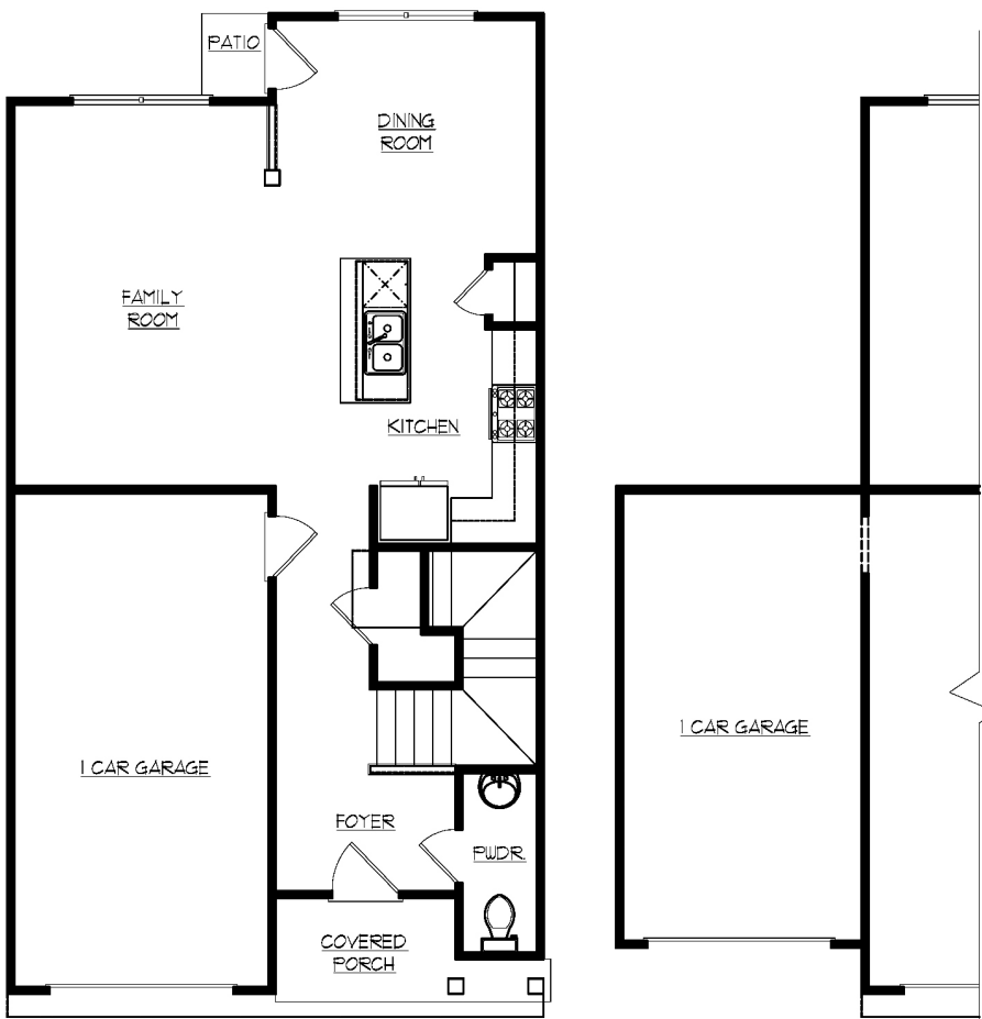
FIRST FLOOR PLAN W/ OPT. 2ND GARAGE
