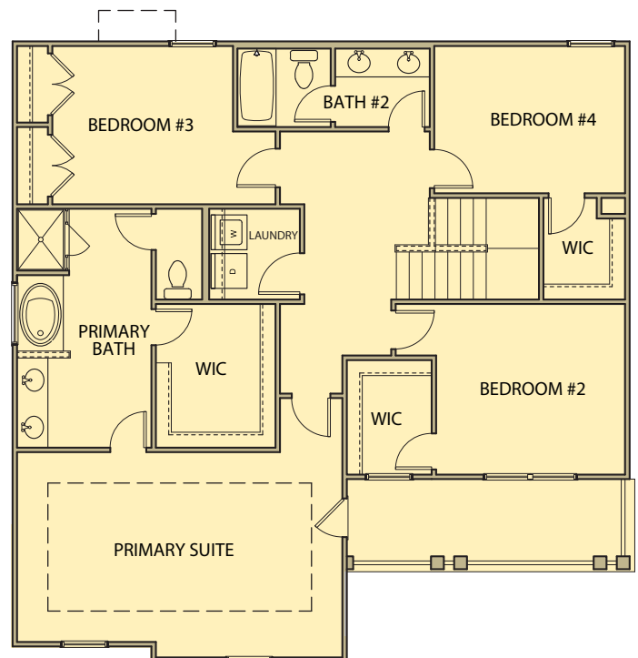
Second Floor (Elevation CC)
