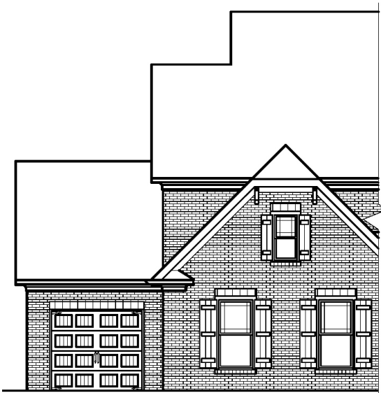
OPT. 3RD CAR GARAGE W/ SIDE ENTRY GARAGE
