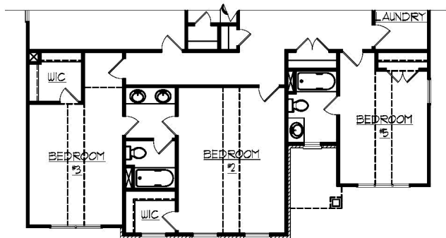
SECOND FLOOR PLAN W/ OPT. BEDROOM #5 & BATH
