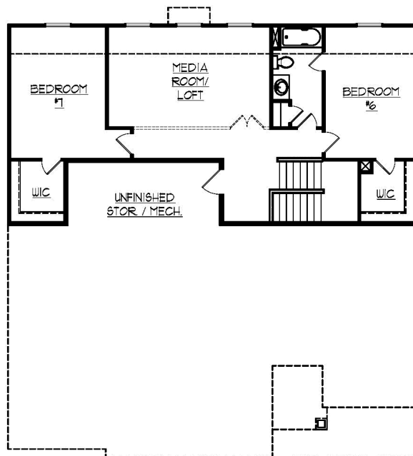
OPT. THIRD FLOOR PLAN
