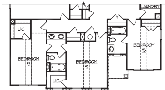
SECOND FLOOR PLAN W/ OPT. BEDROOM #5 & BATH
