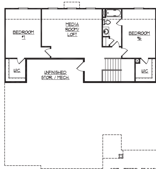
OPT. THIRD FLOOR PLAN
