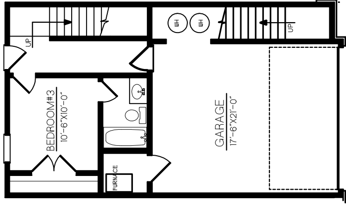
THE BIRCH BASEMENT PLAN
