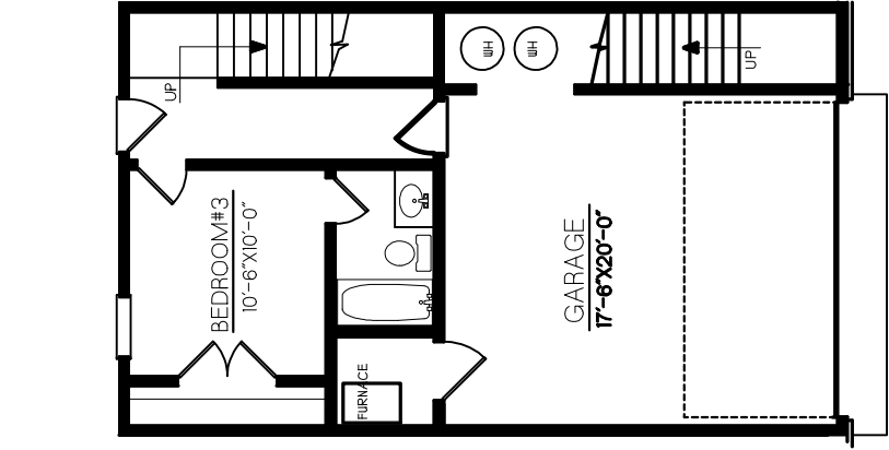
THE REDWOOD BASEMENT PLAN
