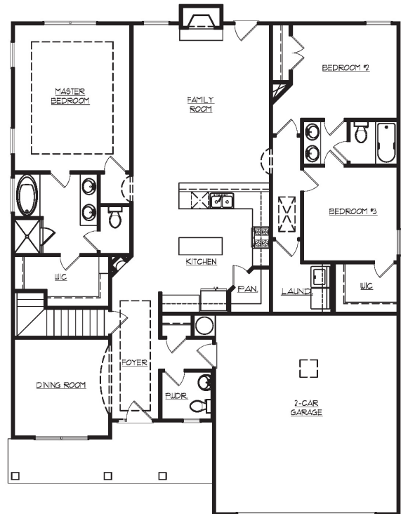
FIRST FLOOR PLAN W/OPTIONAL BASEMENT
