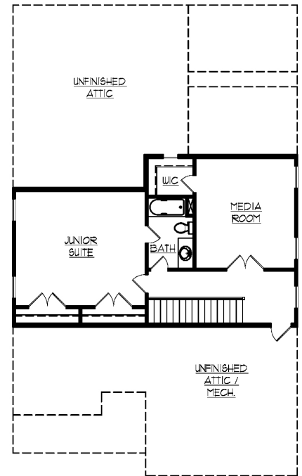
OPT. SECOND FLOOR PLAN W/ MEDIA ROOM
