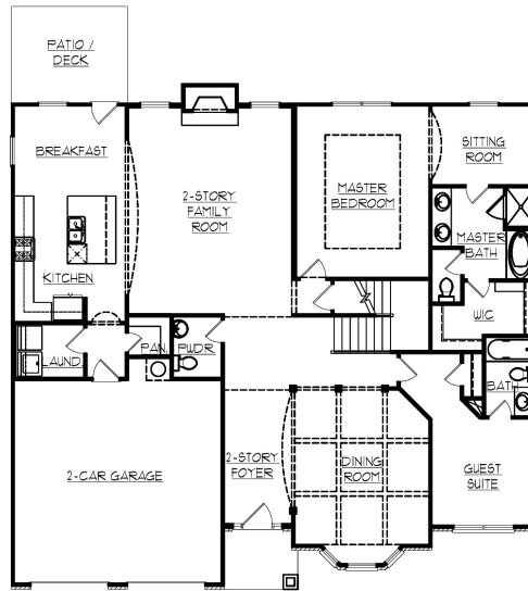
FIRST FLOOR WITH OPTIONAL GUEST SUITE
