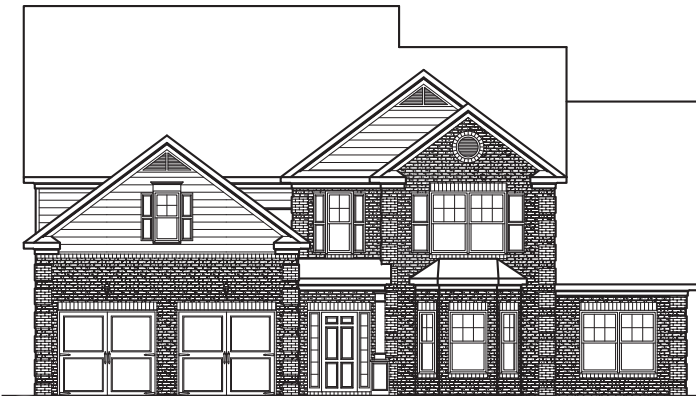
FRONT ELEVATION "A"
