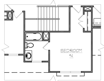
SECOND FLOOR PLAN W/ OPT. BATH BED #4
