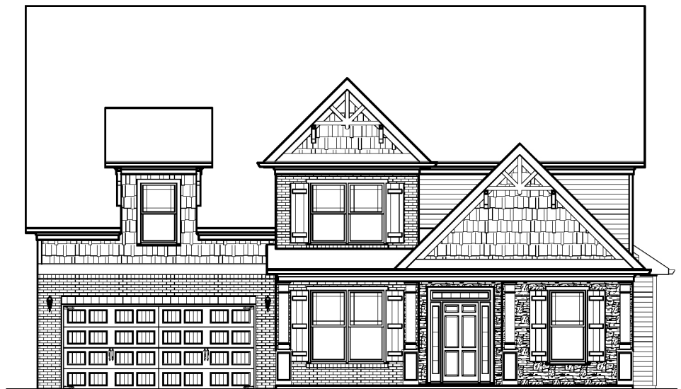
FRONT ELEVATION "CLASSIC"
