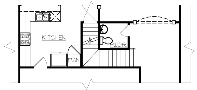
FIRST FLOOR PLAN W/ OPT. BASEMENT
